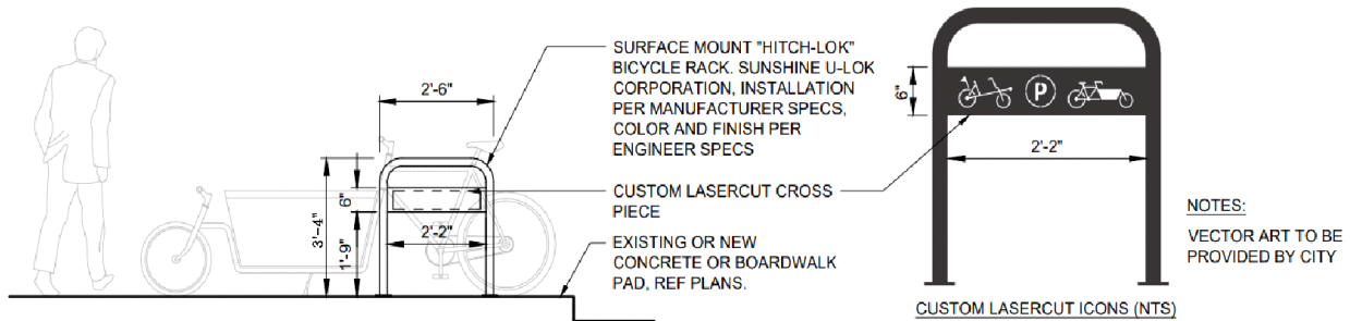
3 BIKE RACK - HITCH CUSTOM CARGO RACK SCALE: 1/2" = 1'-0" XREF
