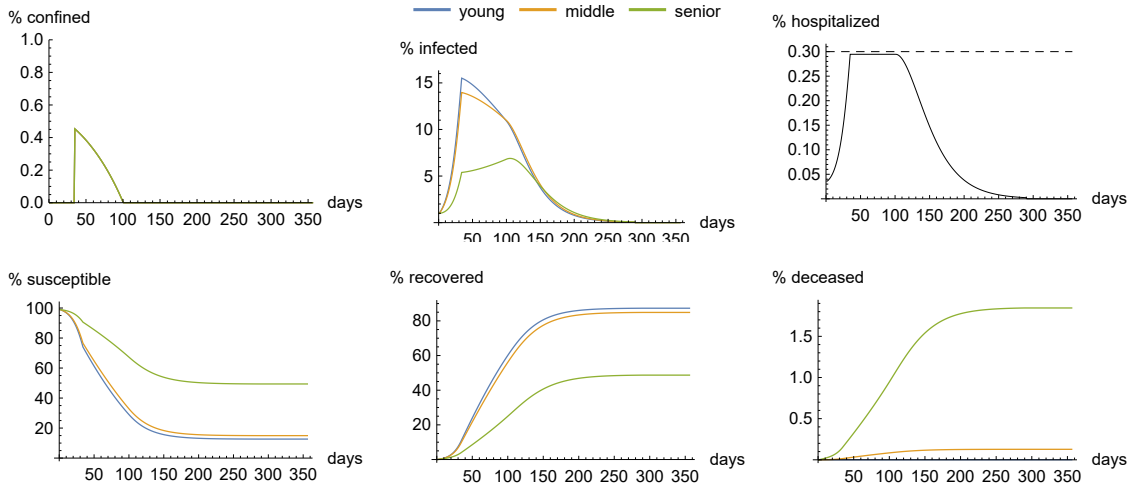
Figure 8: Optimal flatten-the-curve strategy: Dynamics of the pandemic under the Micro-Spiro-Weibull strategy of minimal daily confinement compatible with the health care capacity constraint.
