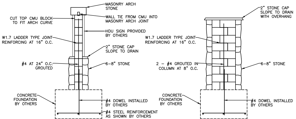
SECTION VIEWS
