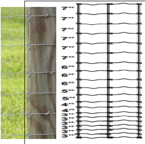
GRADUATED WOVEN WIRE & STAPLES REFERENCE POINTS
