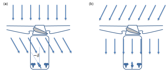
Figure 2. Illustration of the simplified flow in front of and behind the rotor. (a) The blade forces the flow to twist and an optimal aligned turbine obtains a flow deflection angle \delta , which needs to be considered in the turbine alignment. (b) A turbine with the wind vane aligned to the rotor axis faces the wind at a certain yaw angle.
