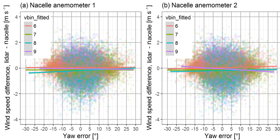
Figure 13. Wind speed difference between a ground-based measurement in front of the turbine and the cup anemometers on the nacelle after the correction with the linear model. The lines represent linear regressions for the respective wind speed bin. The dependency on yaw error is significantly reduced.
