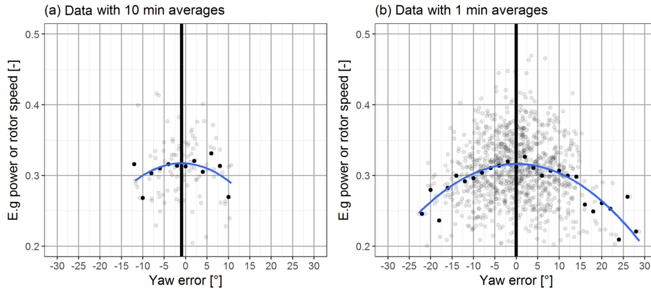
Figure 6. Example of the determination of the best operational alignment. The data are simulated with the same distribution derived from Fig. 5 with a mean yaw error of 0^\circ and 1000 min duration. Normalized active power or rotor speed for a specific wind speed bin as a function of the yaw error. The transparent dots are values with an averaging period of 1 min (b) and 10 min (a). The solid dots represent the yaw error bin averages. The curved line is a second-order polynomial fit with the method of least squares. The maximum is highlighted with a vertical bar. Data with averages of 10 min periods (a) show less curvature than data with 1 min (b), which can lead to small deviations for the derived mean yaw error.
