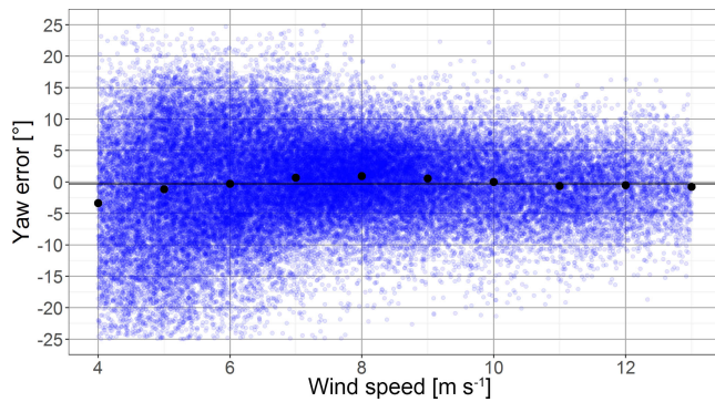
Figure 3. Turbine alignment check based on the comparison of a ground-based lidar wind direction measured with the velocity azimuth display (VAD) technique and the turbine wind direction (yaw error) plotted against the wind speed. The median yaw error per wind speed bin is indicated by the black dots and the overall mean by a horizontal line. Data are averages of 1 min periods and obtained from the experimental setup described in Sect. 2.3.
