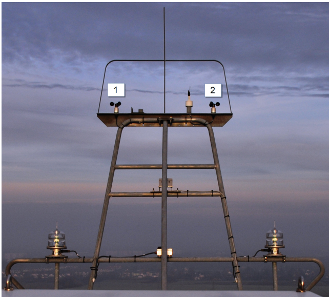
Figure 7. Typical layout of a nacelle-mounted met mast. Lightning rod, two cup anemometers (1 + 2), one wind vane and aviation lights.
