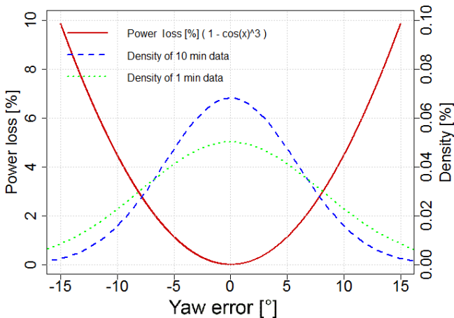
Figure 5. The red solid line indicates the power loss as a function of the yaw error, assuming the cubic-cosine relationship. The dotted and dashed lines represent data densities, fitted with Gaussian distributions. Both lines are based on the same raw data with 1 Hz resolution, but the green dotted distribution shows the data with an averaging period of 1 min and the blue dashed line is the data with 10 min averaging. Higher data resolution (e.g., 1 min data instead of 10 min data) has a larger standard deviation and therefore provides more data points at extreme conditions where the effects of power losses are more pronounced. This enables better evaluation of the best point of operation.
