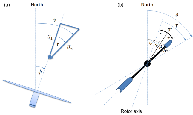
Figure 1. Definition of angles. (a) The angle between the rotor axis and the true north is called the nacelle position \phi . The angle between the true wind direction ( \vartheta ) U_\infty and its component perpendicular to the rotor plane U_\perp is denoted as yaw error \gamma . (b) The wind vane is located behind the rotor. Its assembly angle \varphi with respect to the rotor axis, the measured value \mu and the flow deflection angle \delta between the wind vane and true wind direction sum up to the yaw error \gamma .
