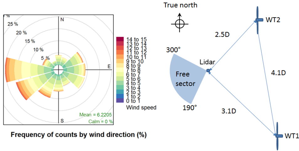
Figure 4. Layout of the test wind farm and frequency distribution of wind speeds by wind direction. Two 2 MW turbines with a rotor diameter of 92 m turbines and a ground-based lidar measuring inflow conditions with the velocity azimuth display technique (VAD) in the free sector are shown.
